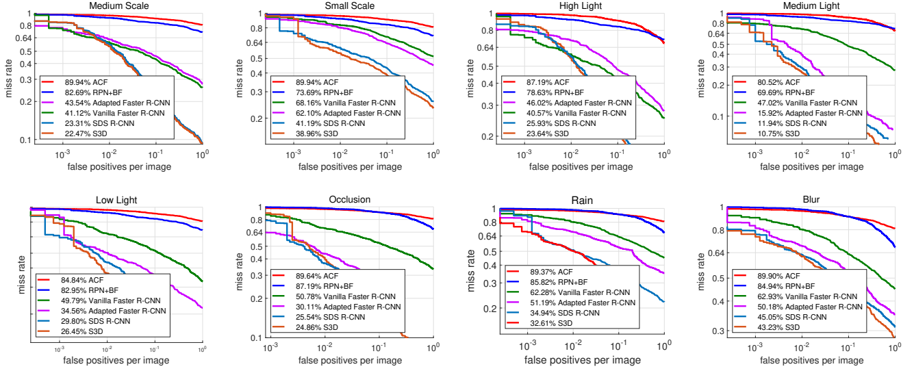
Figure 3: Miss rates versus false positives of existing classical algorithms on different settings of NightSurveillance dataset. Lower curve means better performance, the legend denotes average miss rate.
