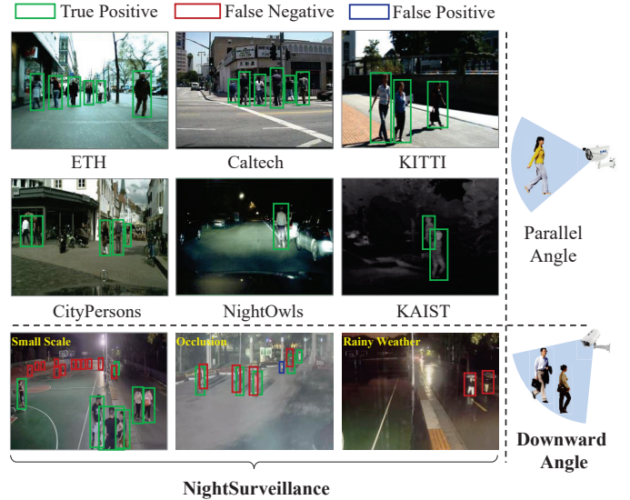
Figure 1: Some typical examples and results of the S3D detector to show the differences of our NightSurveillance dataset and existing datasets. Existing datasets include ETH, Caltech, KITTI, CityPersons, NightOwls, and KAIST. For our datasets, we show some real-world challenging conditions, such as small scale, occlusion, and rainy weather.
